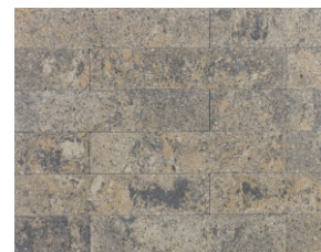
pyrite
